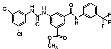
Compound # 5
